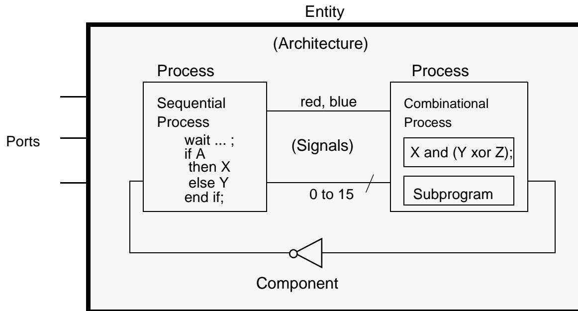
Figure 1-1: VHDL Hardware Model
