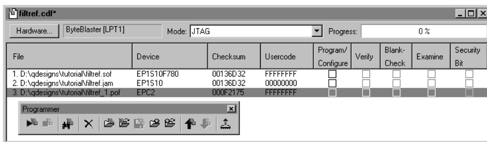
Figure 2. Programmer Window
