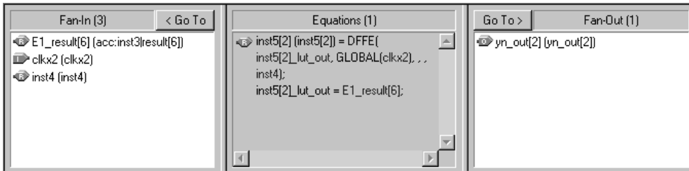
Figure 2. Equations Window
