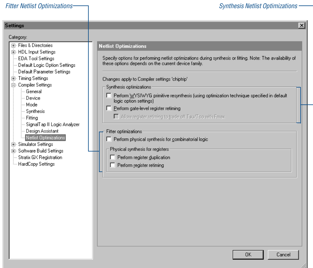
Figure 3. Netlist Optimizations
