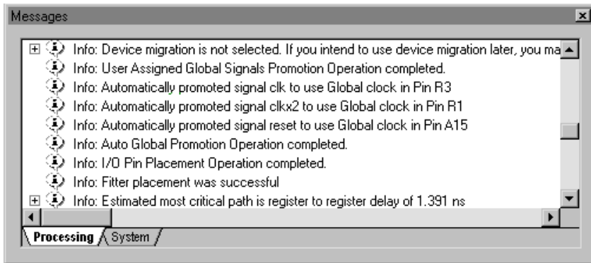
Figure 3. Messages Window
